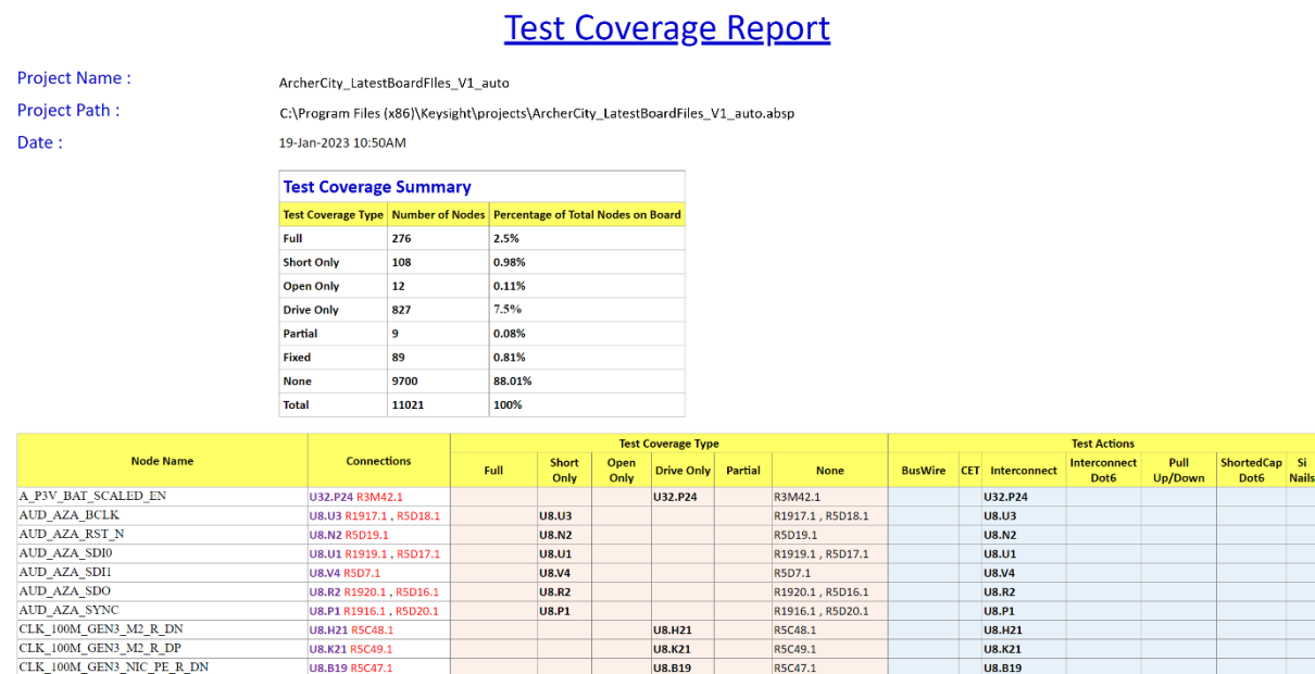
Figure 6. Test coverage report for test coverage classification
