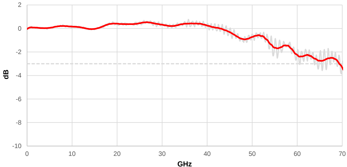
Figure 5. Frequency response at front panel output, measured at sample rate of 128 GSa/s, and 1 Vpp,diff amplitude. Sin(x)/x roll-off mathematically compensated. Red: Savitzky–Golay filters polynomial fit, window size: 5%, grey: measured data.
