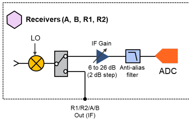
Receiver block diagram (port 1 and 2)
