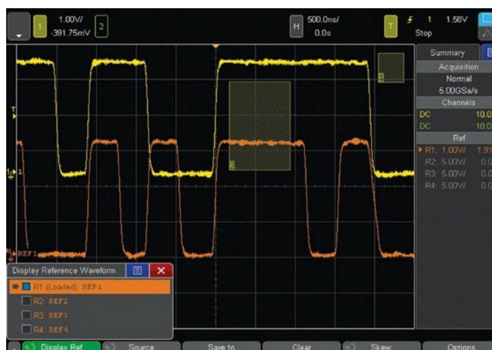
Figure 33. Store and recall up to four reference waveforms.
