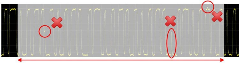
Figure 4. Other vendor's oscilloscope with 50,000 waveforms/second. A long dead time (gray area) decreases your chances of capturing infrequent events.
