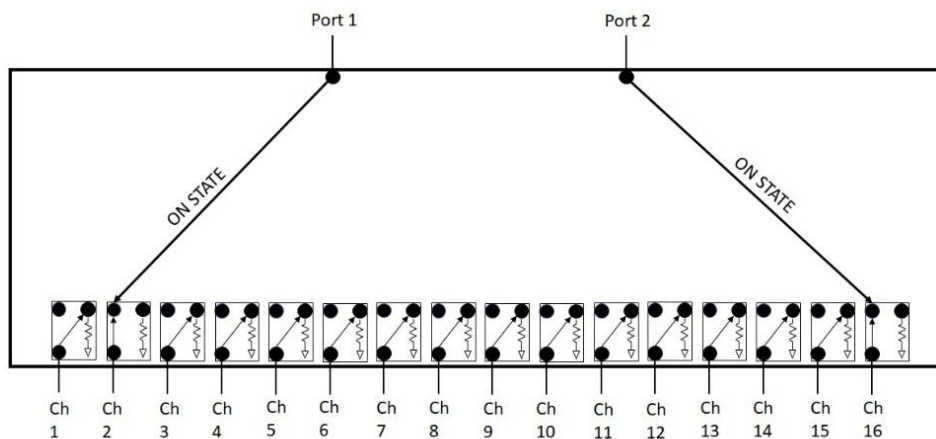
Figure 2. Simplified block diagram of 2X16 switch matrix
