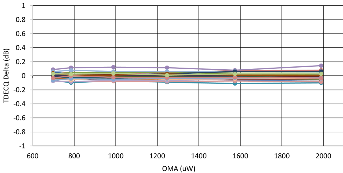
Figure 4. 106.25 GBd TDECQ ChanA Delta from ChanB (Each line on the graph represents the difference in TDECQ measurement results between Channel A and Channel B of one N1093 unit.)
