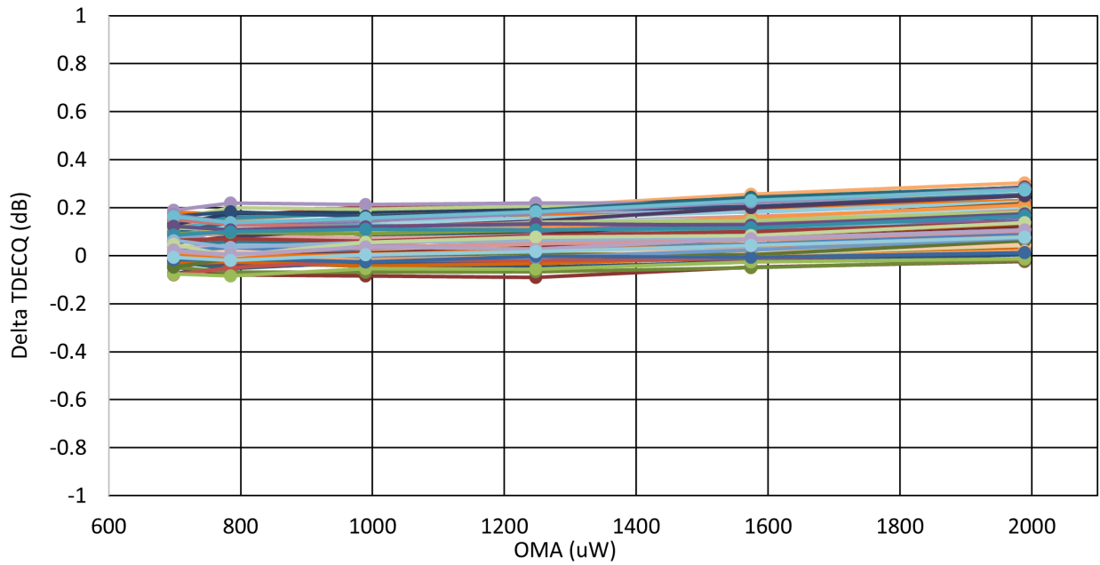
Figure 3. 106.25 GBd TDECQ Delta from TDECQ-Reference (Each line on the graph represents one N1093 channel measured relative to the TDECQ reference.)
