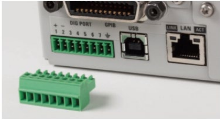
Figure 10. Digital control port on the rear panel
